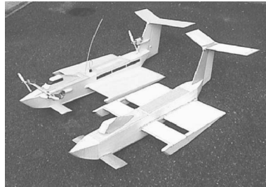
Figure 13 : MK5 with MK6 under construction to test 'Through-Wing' flaps.
