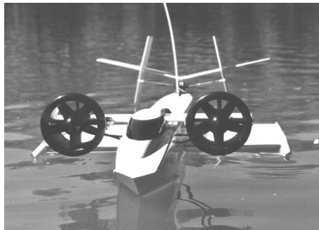
Figure 6 : The streamlined, thin-winged MK3 model
